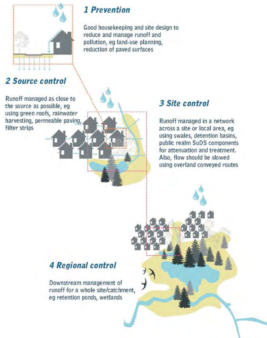
Figure 1.6.1 The SuDS management train (CIRIA, 2010)
