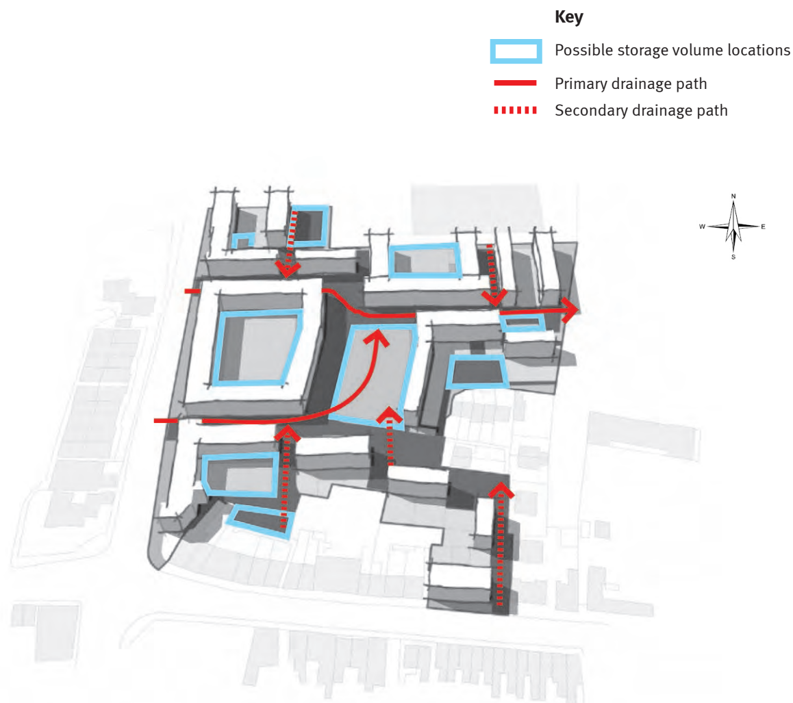
Figure 4.2.4.2: Initial assessment of flow routes and potential storage volumes
