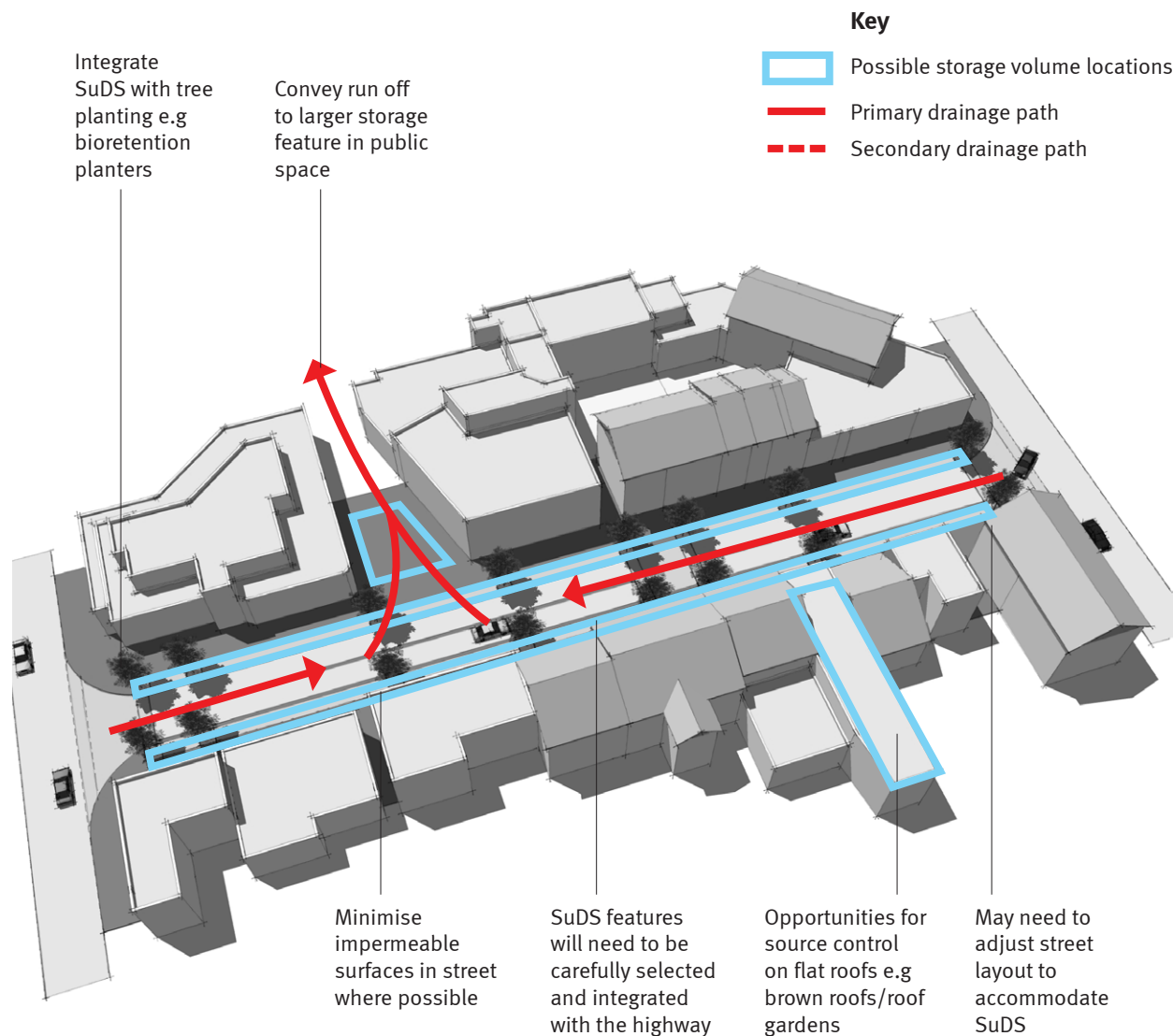
Figure 4.2.3.2: Initial assessment of flow routes and potential storage volumes
