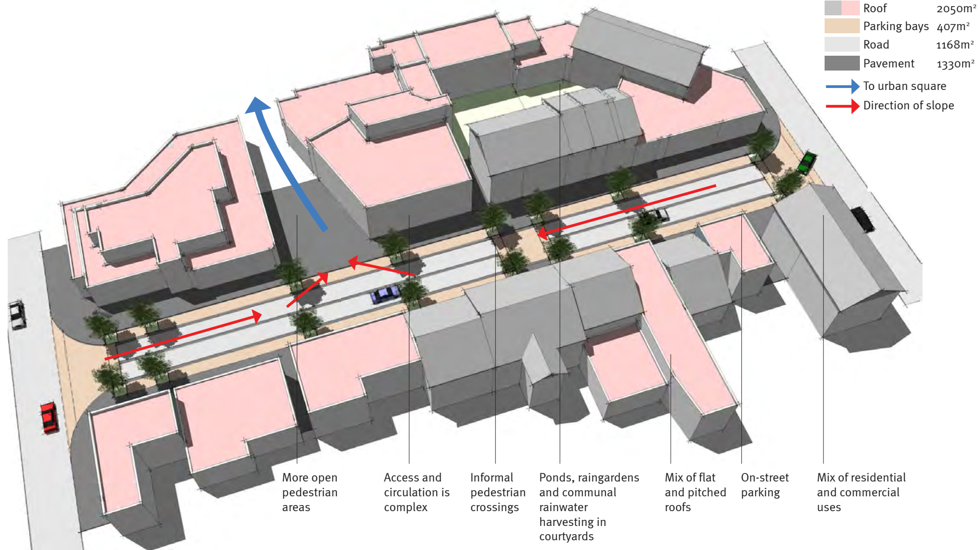
Figure 4.2.3.1: Analysis of proposed development
